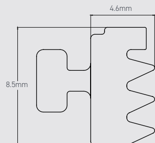
4mm Inner (Bead) Glazing Seal A-07698
