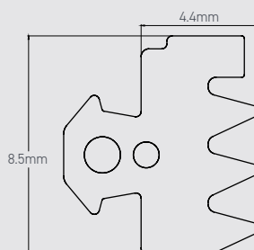
4mm Inner (Frame) Glazing Seal A-07697
